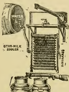
Star Milk Cooler.
